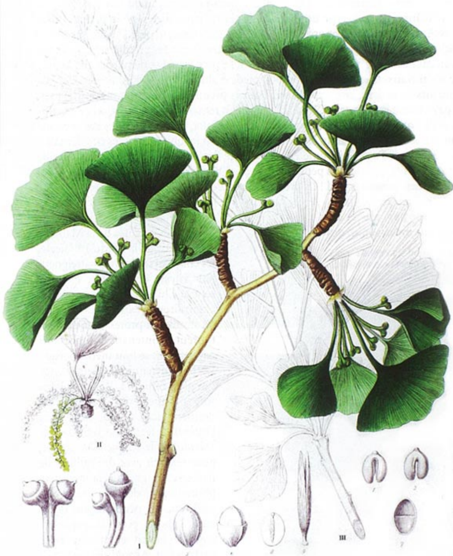
SALISBURIA adiantifolia .
